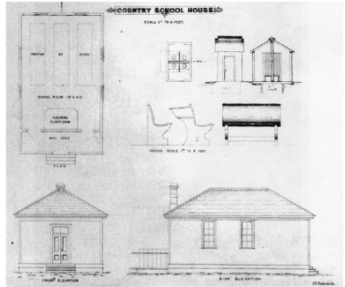
Country School House Plan, Department of Land &amp; Works, BCA 54-4-89
