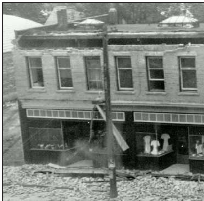
Fig. 2.8: Port Alberni Bank of Montreal earthquake damage, 1946. (Source: CDM)
