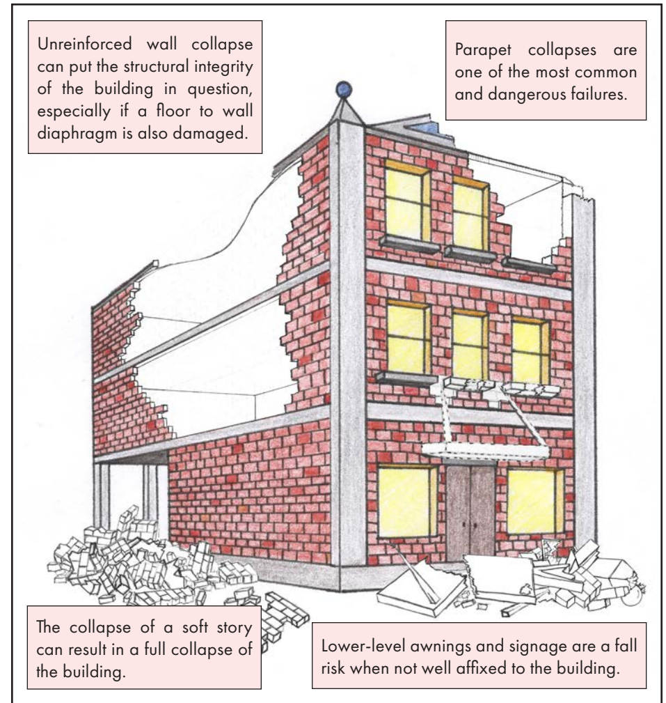
Fig. 2.11: Illustration of some of the common failure and damage potentially experienced by existing buildings during a seismic event, particularly heritage buildings. (Source: Ian Babbitt)
