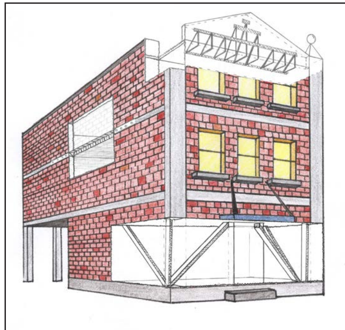
Fig. 3.3: Illustration of some of the different seismic upgrading options available. (Source: Ian Babbitt)
