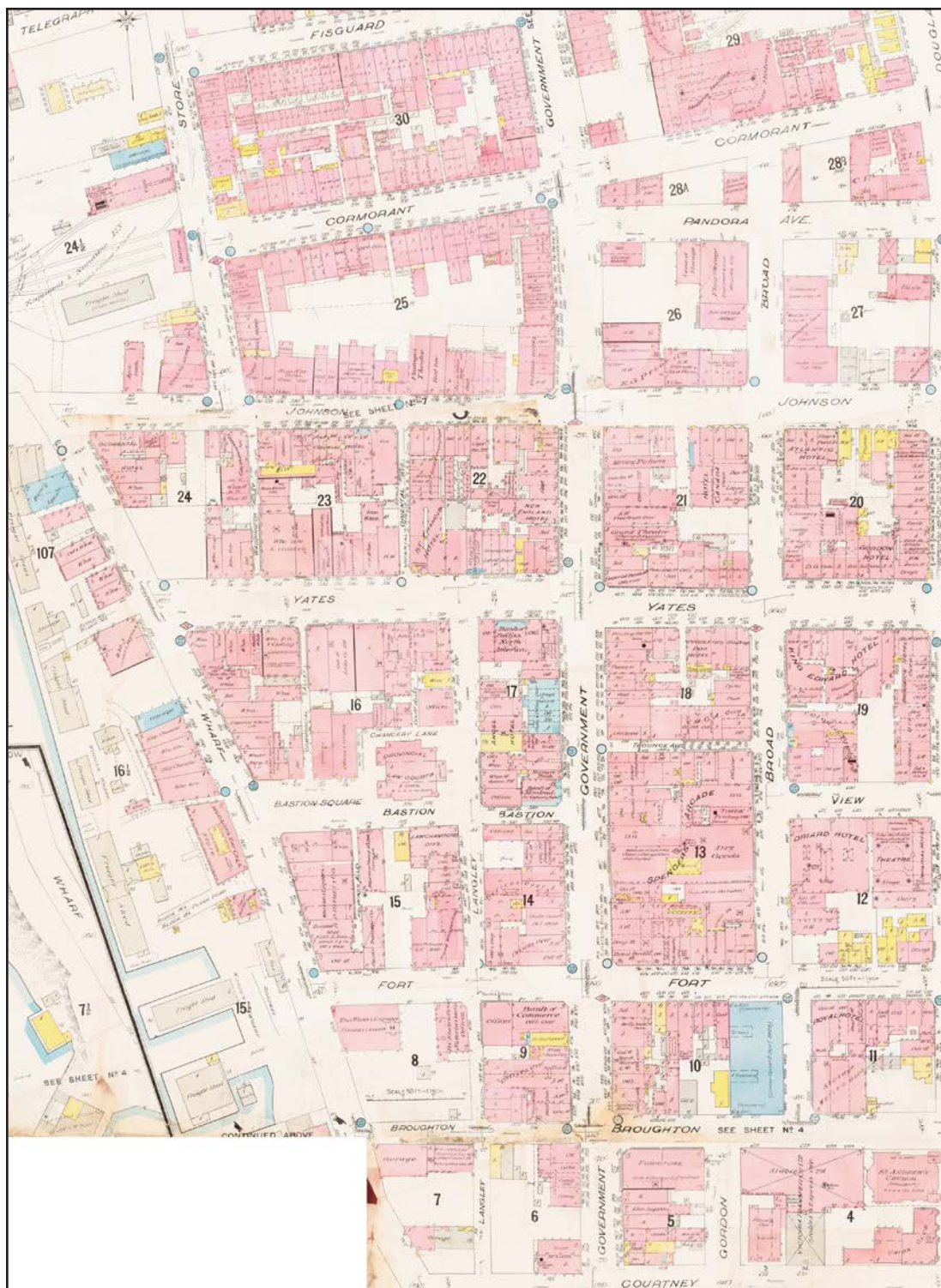
Fig. 4.2: A compilation of fire insurance plan sheets from 1903, showing the various downtown buildings at that time, illustrating their material of construction. Blue denotes stone, red denotes brick and yellow denotes wood. Note the abundant use of brick for this area, many of which still stand today as heritage-registered or heritage-designated buildings. (Source: UVic Vault)
