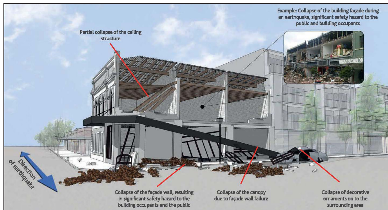
Fig. 5.22: Illustration showing the other direction of earthquake forces acting on a building, with additional example damage. (Source: Auckland Council 2017, p. 25)
