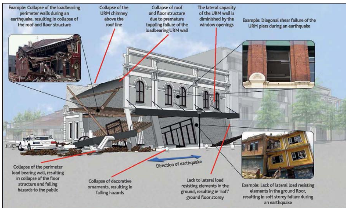
Fig. 5.21: Illustration showing one direction of earthquake forces acting on a building, with example damage. (Source: Auckland Council 2017, p. 24)
