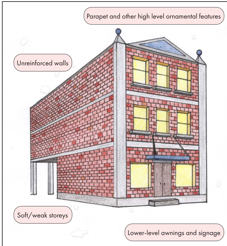
Fig. 2.10: Illustration of a heritage building with some of its potential vulnerabilities pinpointed. (Source: Ian Babbitt)
